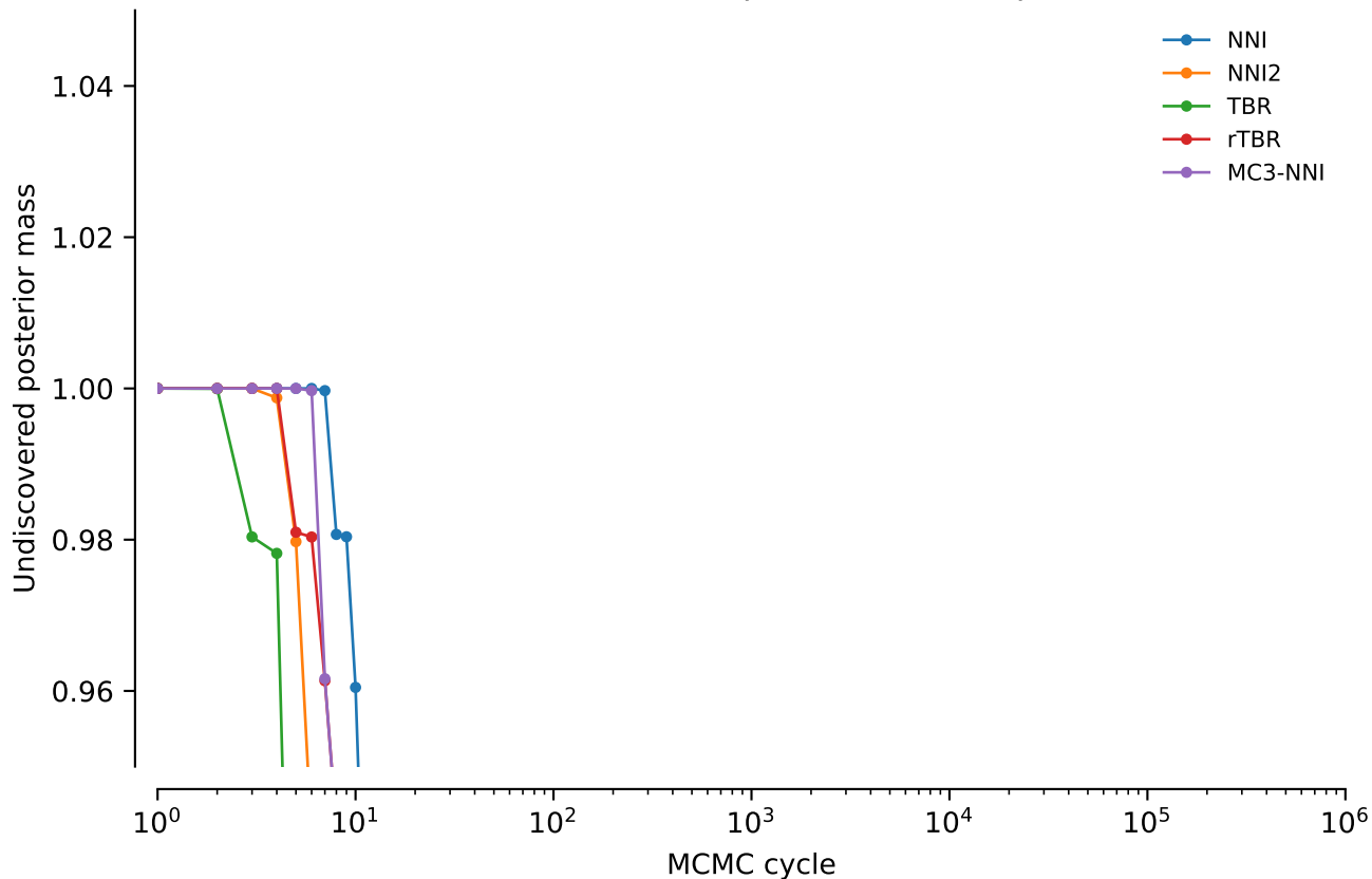
vert.coi.tw5: Undiscovered posterior mass: power = 0.2
