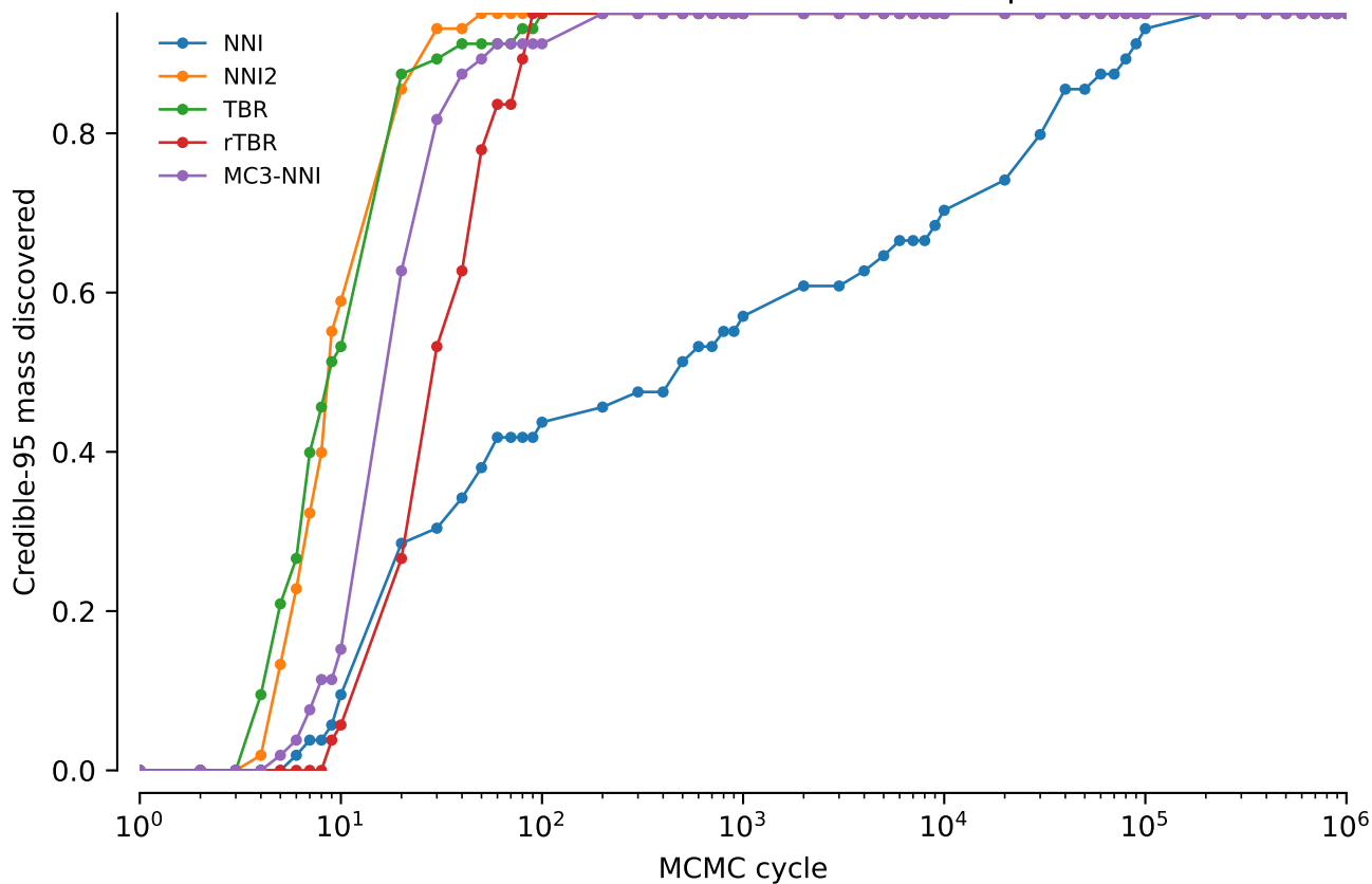
vert.coi.tw5: Credible-95 mass discovered: power = 0.3
