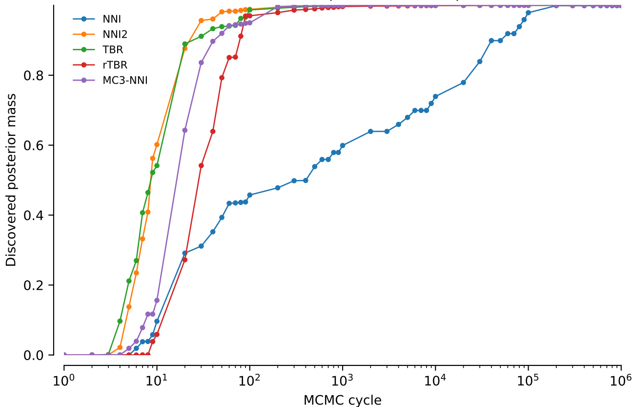
vert.coi.tw5: Discovered posterior mass: power = 0.3
