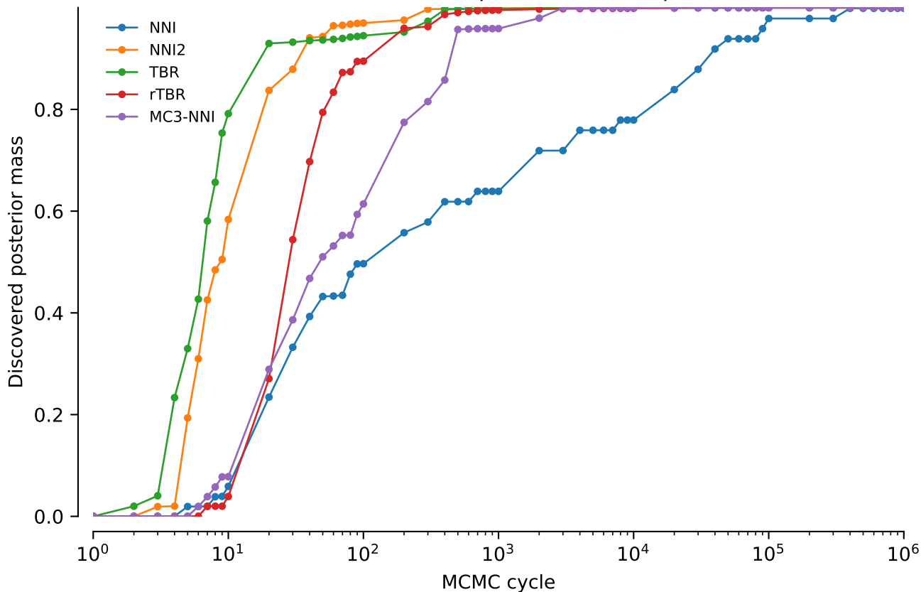
vert.coi.tw5: Discovered posterior mass: power = 0.4
