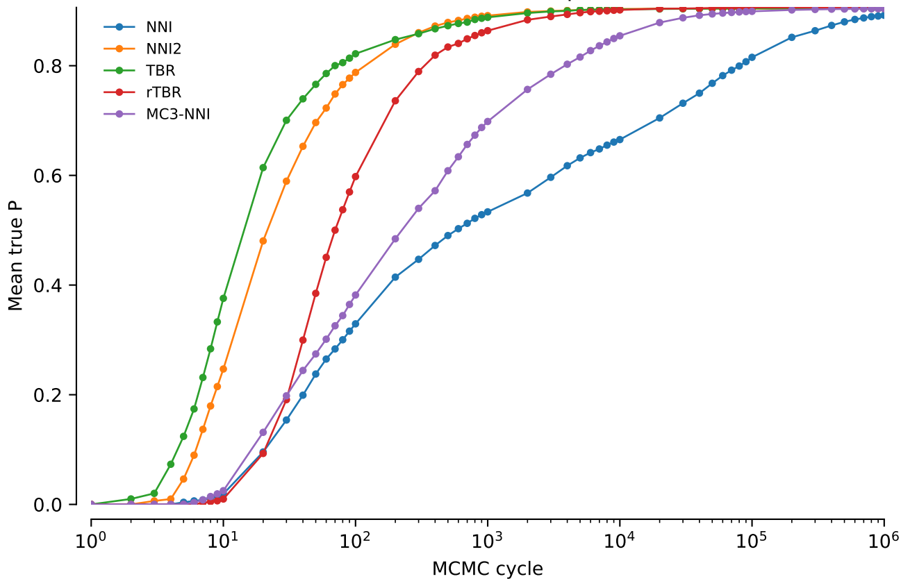
vert.coi.tw5: Mean true P: power = 0.4
