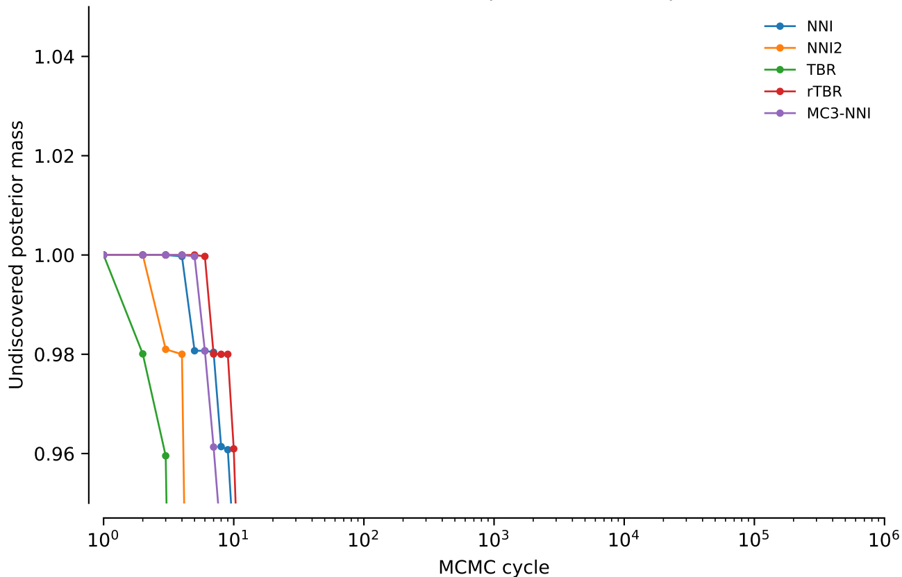
vert.coi.tw5: Undiscovered posterior mass: power = 0.4
