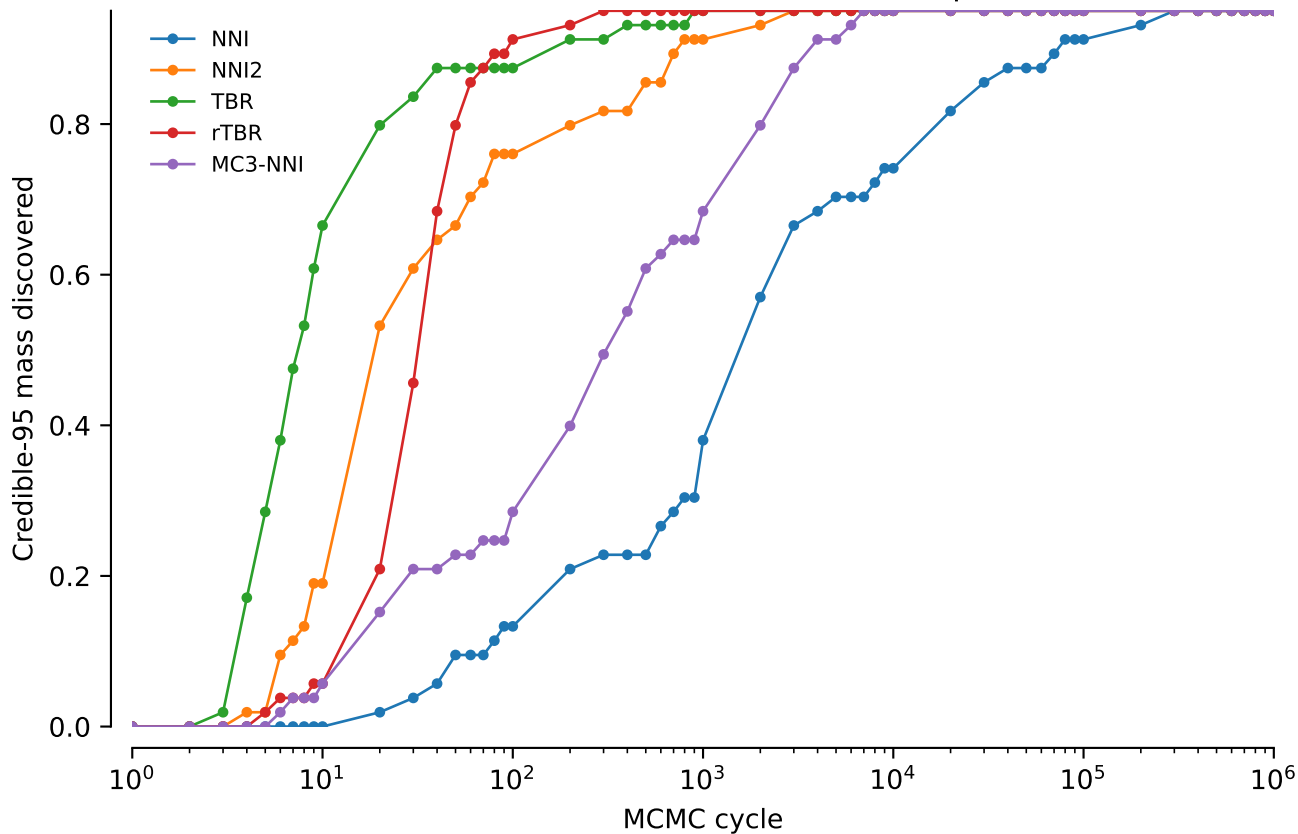
vert.coi.tw5: Credible-95 mass discovered: power = 0.5
