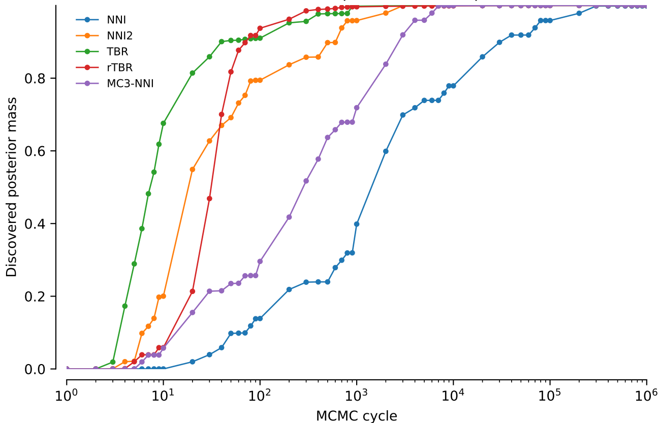
vert.coi.tw5: Discovered posterior mass: power = 0.5
