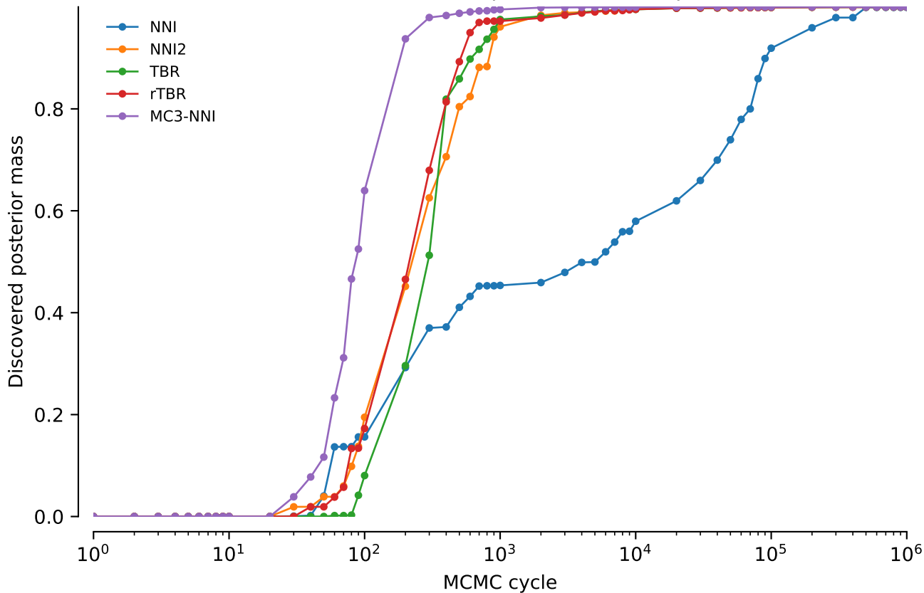
vert.coi.tw5: Discovered posterior mass: power = 0
