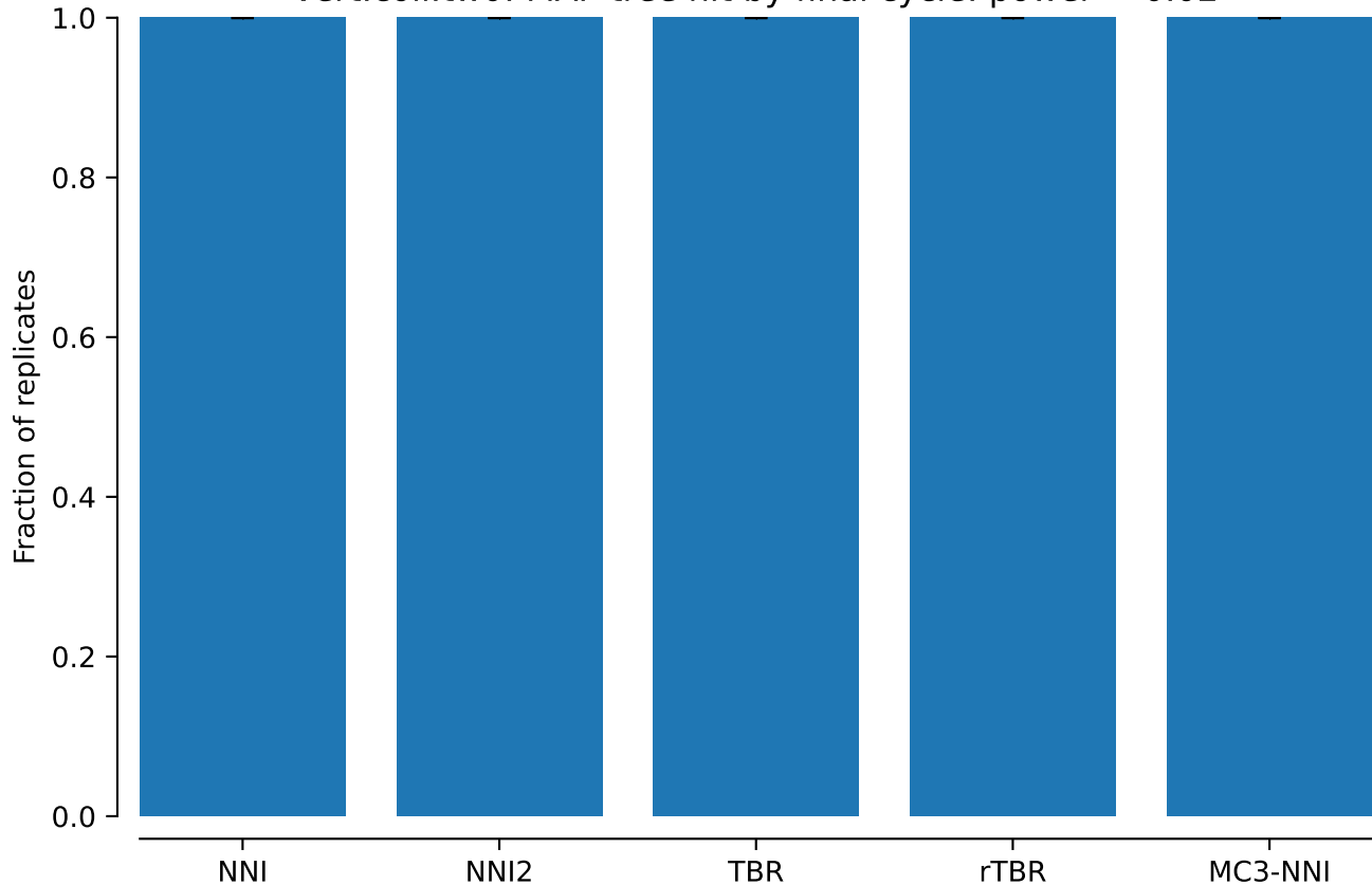
vert.coii.tw0: MAP tree hit by final cycle: power = 0.02
