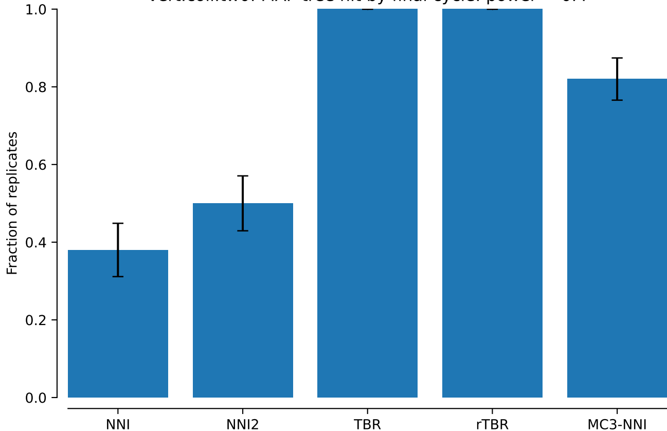
vert.coii.tw0: MAP tree hit by final cycle: power = 0.4
