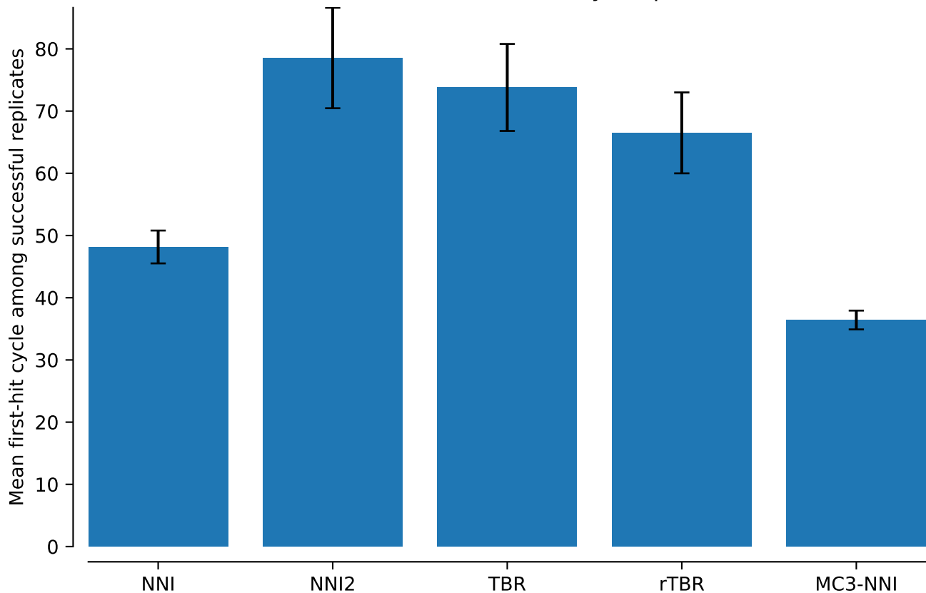
vert.coii.tw0: Mean MAP first-hit cycle: power = 0.02
