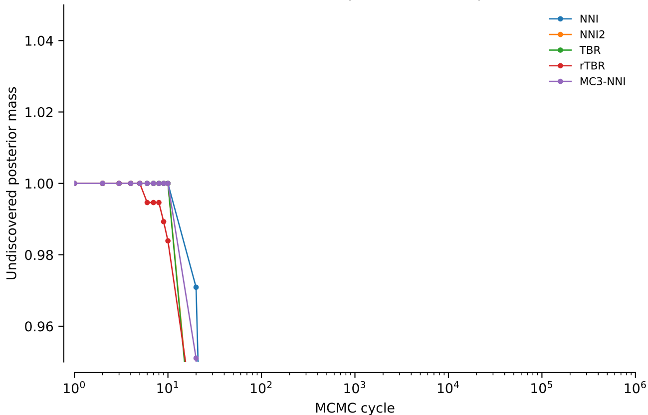
vert.coii.tw0: Undiscovered posterior mass: power = 0.02
