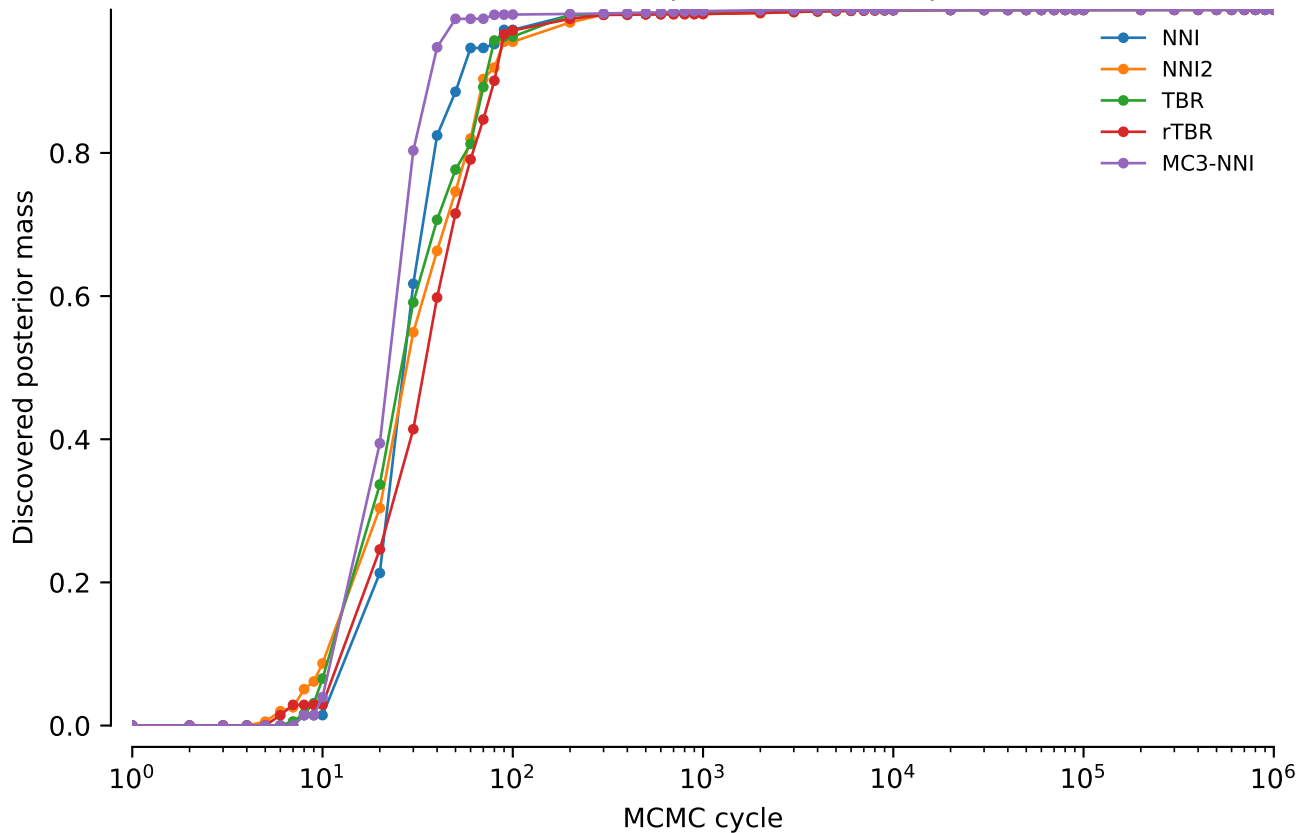
vert.coii.tw0: Discovered posterior mass: power = 0.05
