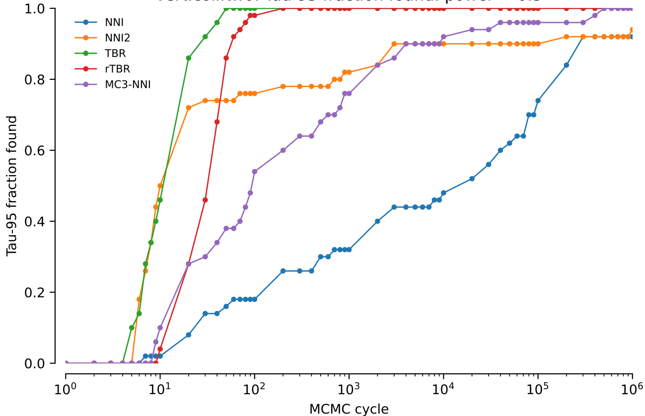
vert.coii.tw0: Tau-95 fraction found: power = 0.3
