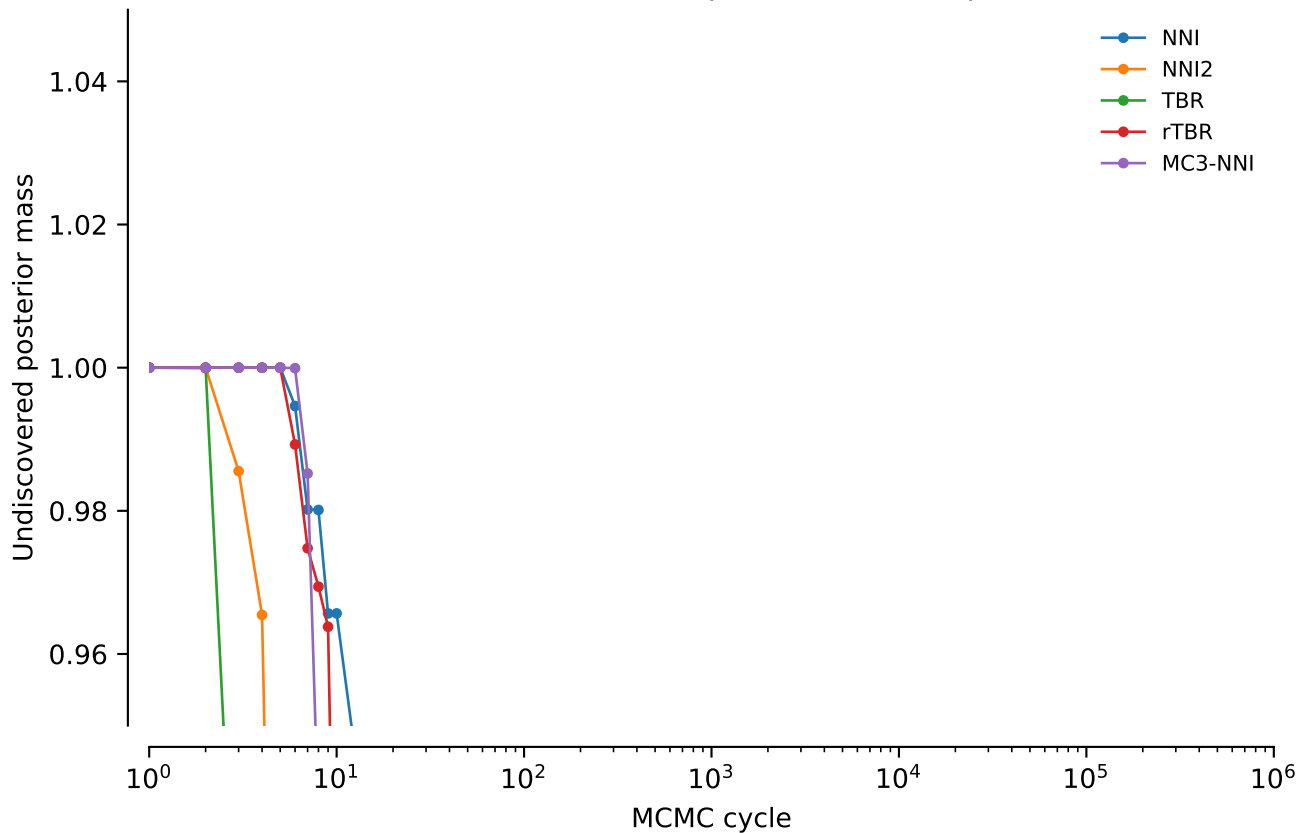
vert.coii.tw0: Undiscovered posterior mass: power = 0.3
