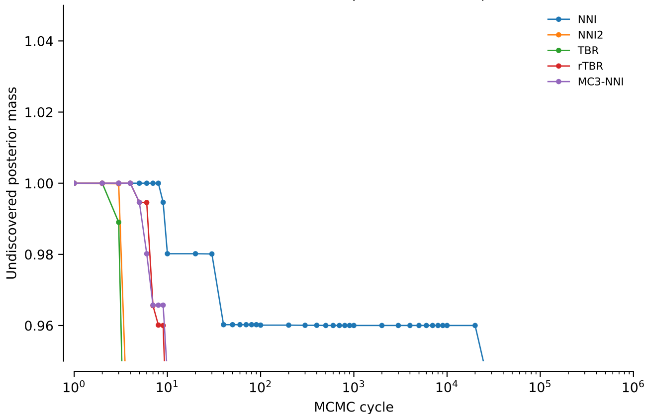
vert.coii.tw0: Undiscovered posterior mass: power = 0.5
