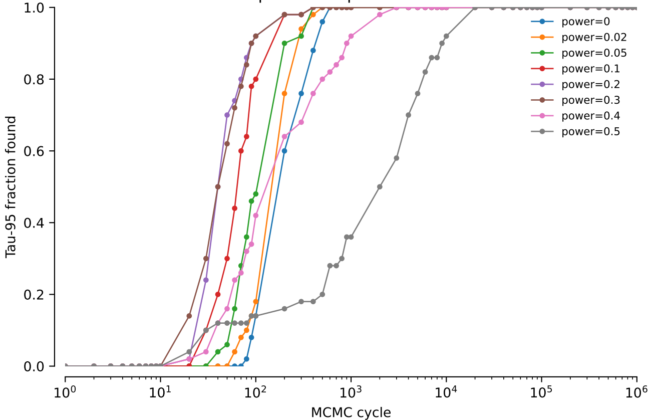
vert.coii.tw5: NNI power comparison: Tau-95 fraction found
