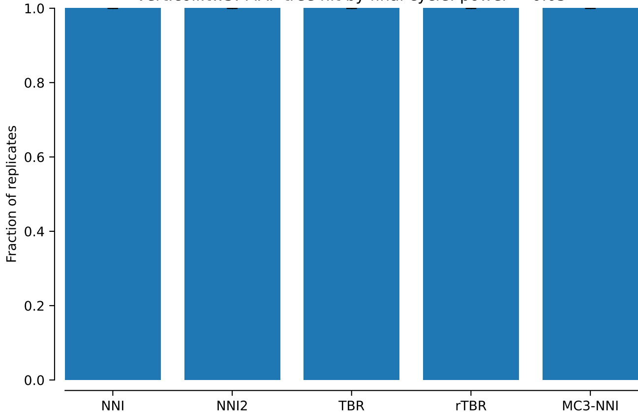
vert.coii.tw5: MAP tree hit by final cycle: power = 0.05
