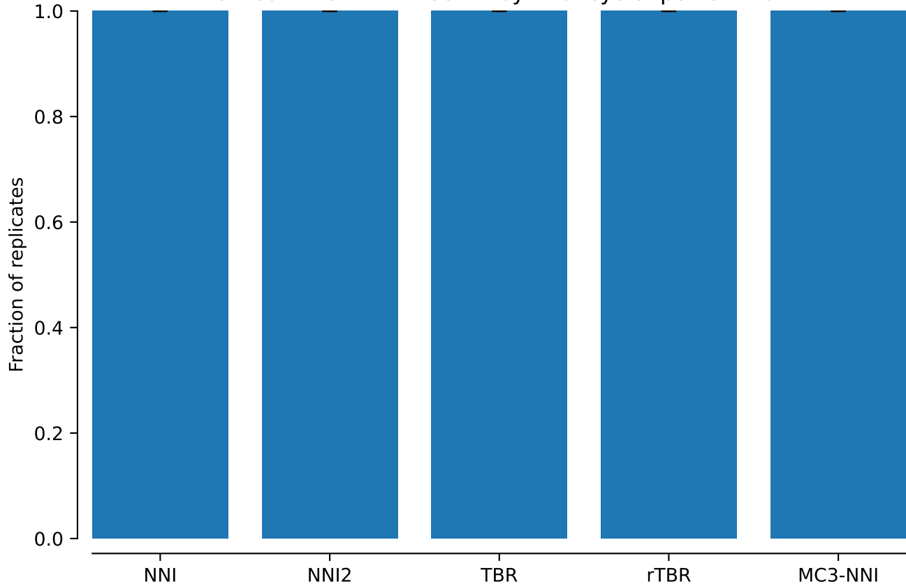
vert.coii.tw5: MAP tree hit by final cycle: power = 0.2
