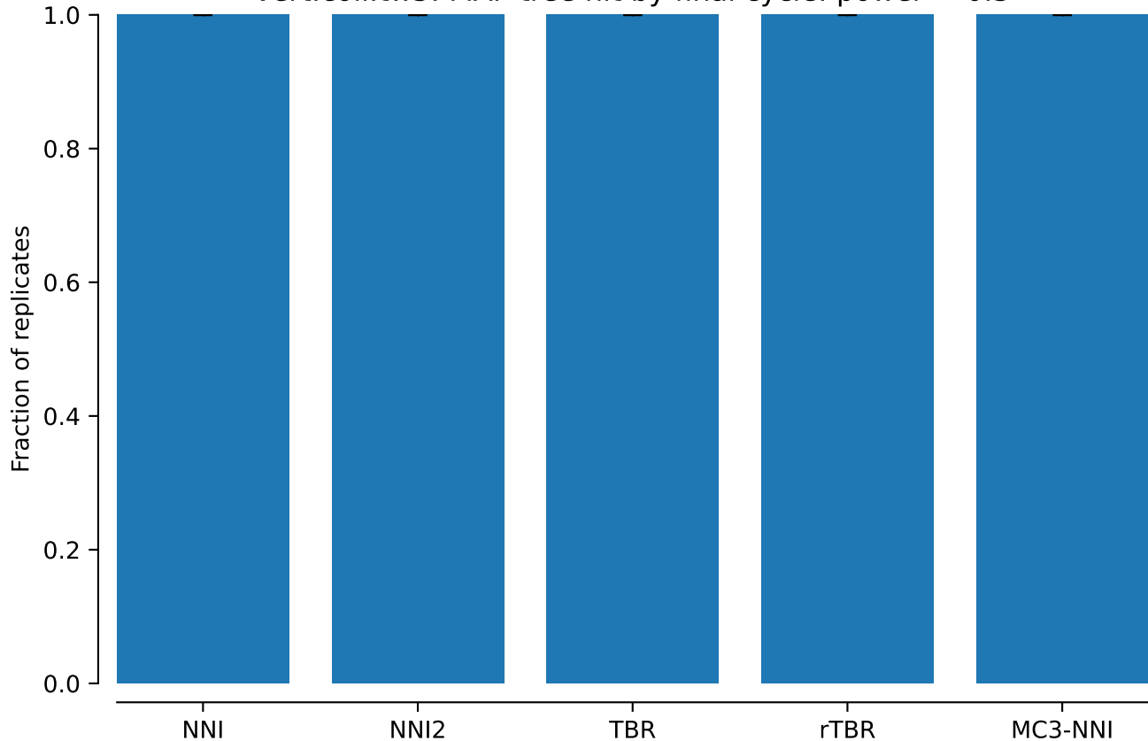
vert.coii.tw5: MAP tree hit by final cycle: power = 0.3
