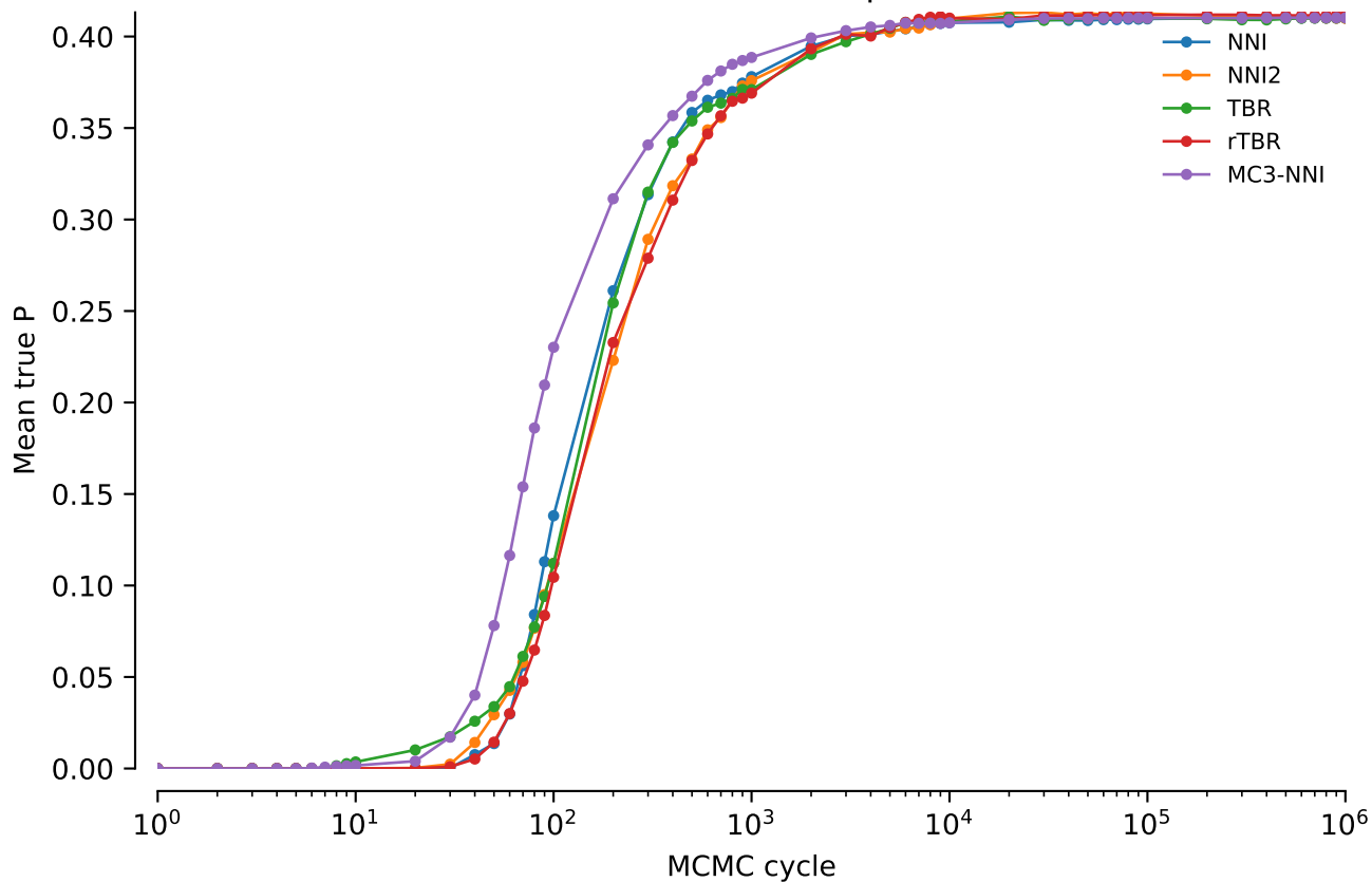
vert.coii.tw5: Mean true P: power = 0.02
