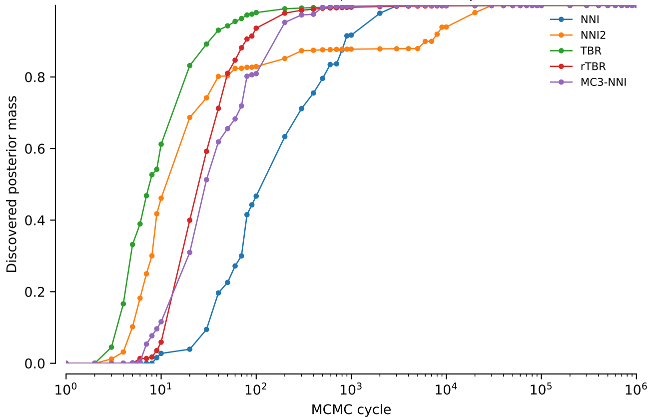
vert.coii.tw5: Discovered posterior mass: power = 0.4
