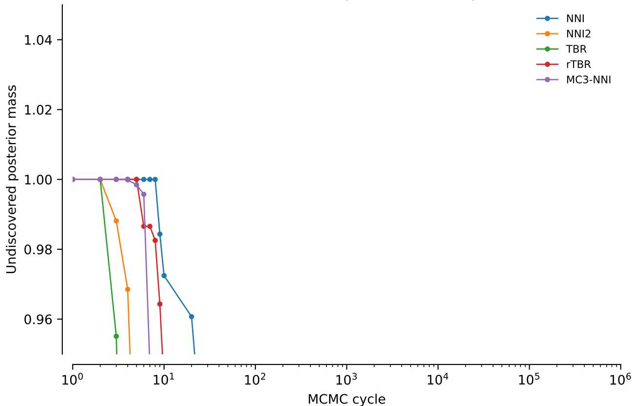
vert.coii.tw5: Undiscovered posterior mass: power = 0.4
