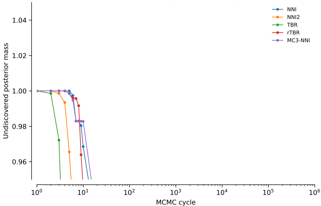
vert.coii.tw5: Undiscovered posterior mass: power = 0.5
