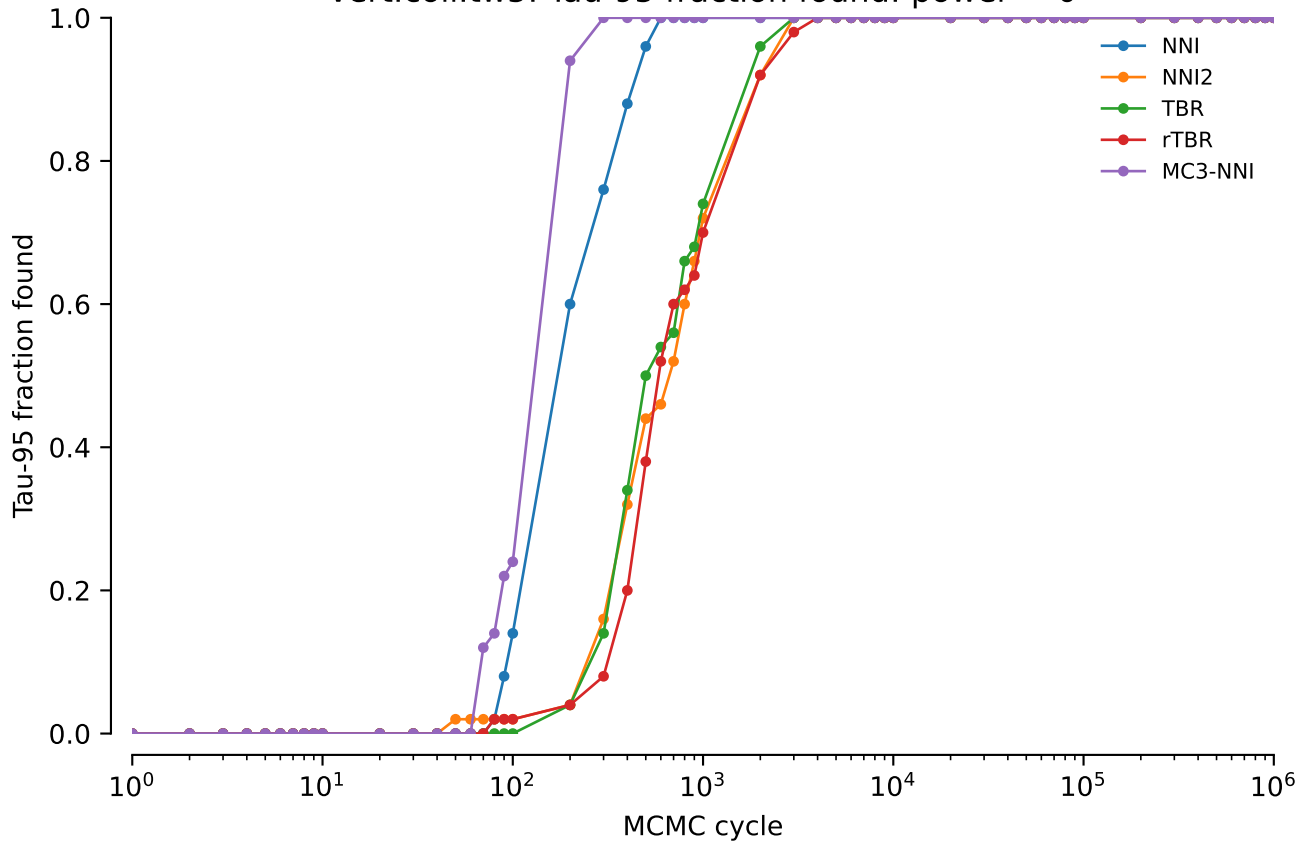
vert.coii.tw5: Tau-95 fraction found: power = 0
