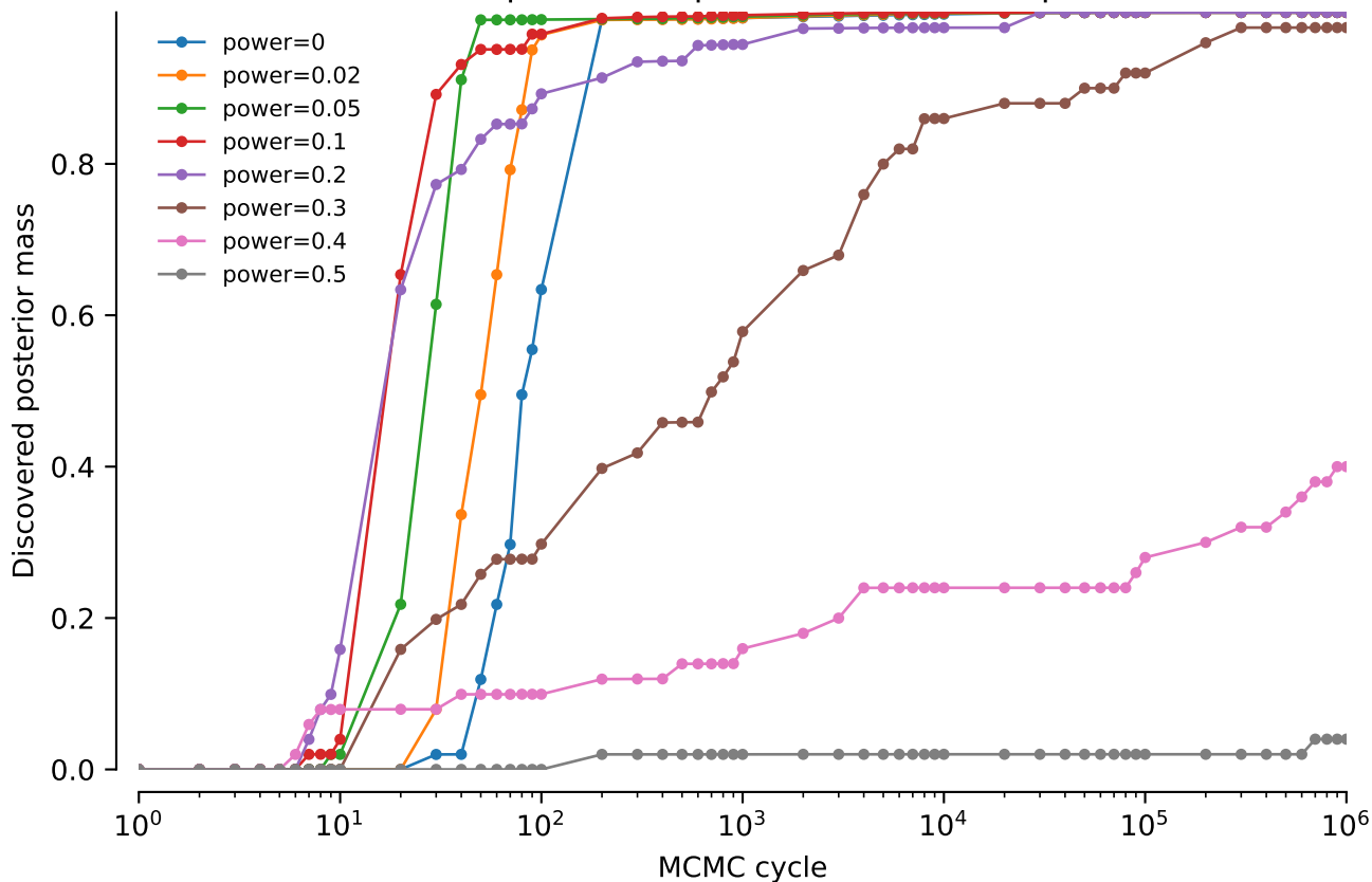
vert.coiii.tw0: NNI power comparison: Discovered posterior mass
