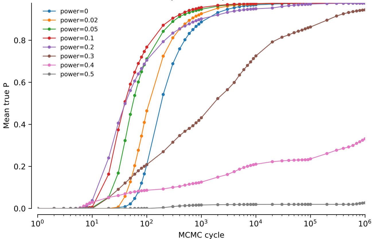
vert.coiii.tw0: NNI power comparison: Mean true P
