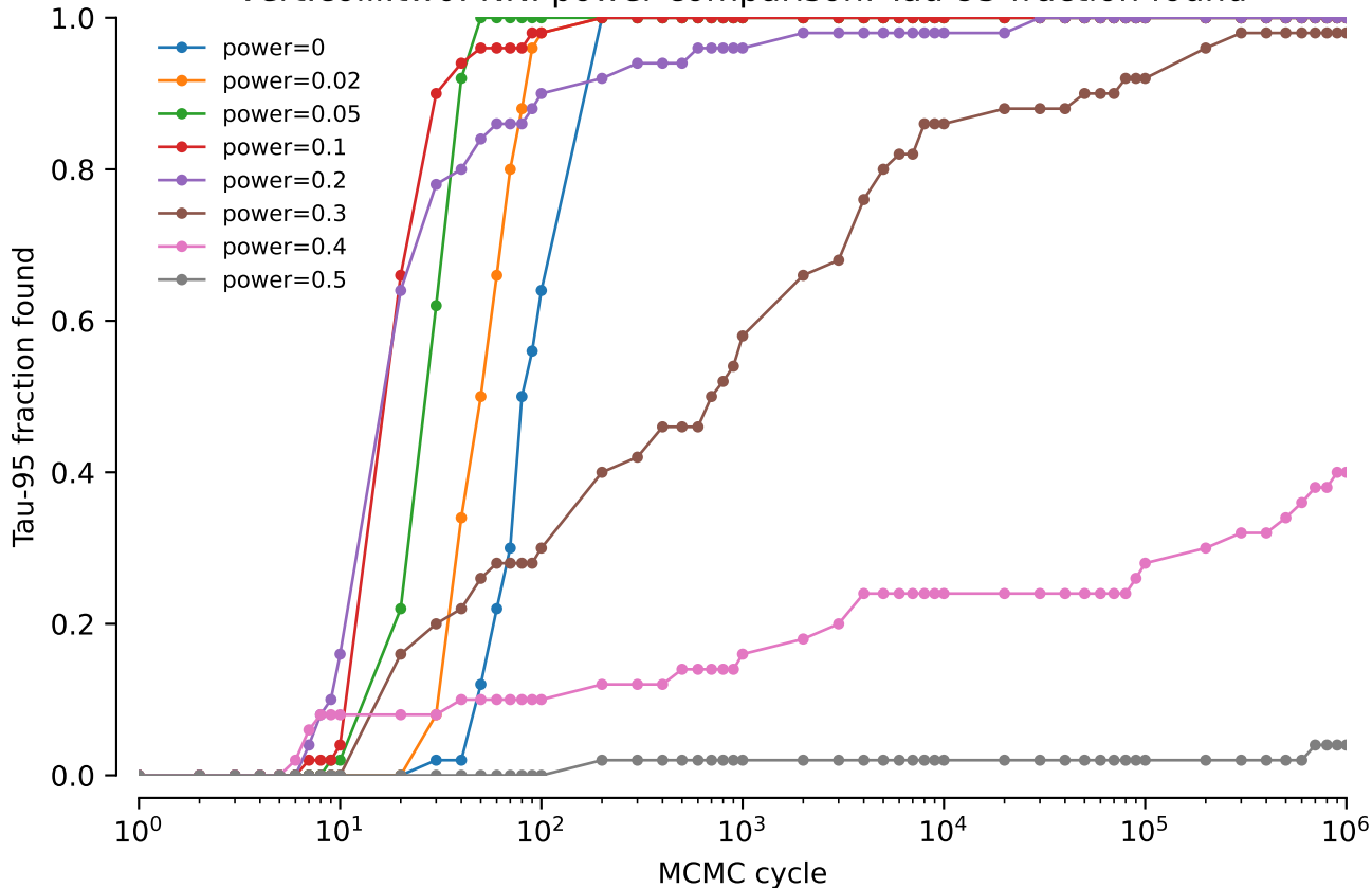
vert.coiii.tw0: NNI power comparison: Tau-95 fraction found
