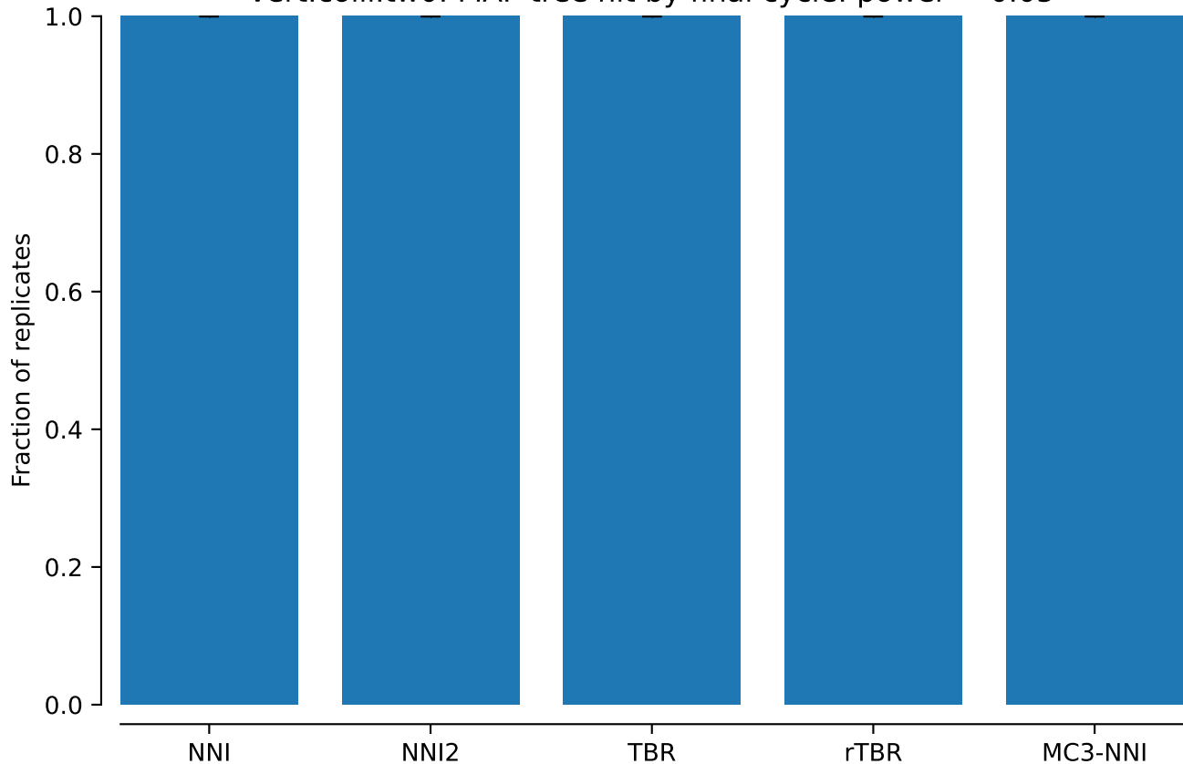
vert.coiii.tw0: MAP tree hit by final cycle: power = 0.05
