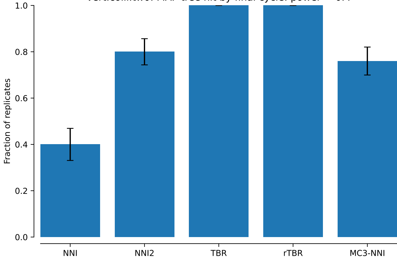
vert.coiii.tw0: MAP tree hit by final cycle: power = 0.4
