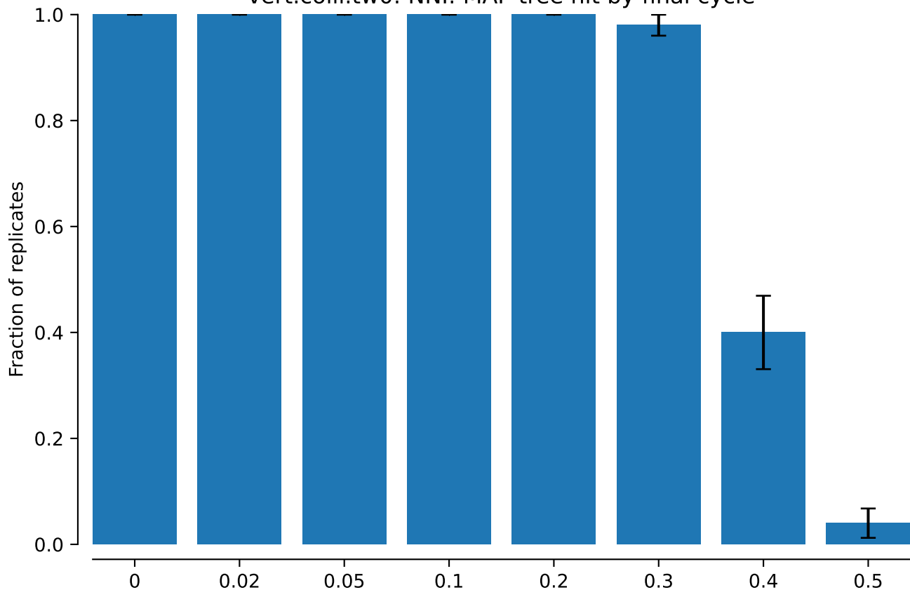
vert.coiii.tw0: NNI: MAP tree hit by final cycle
