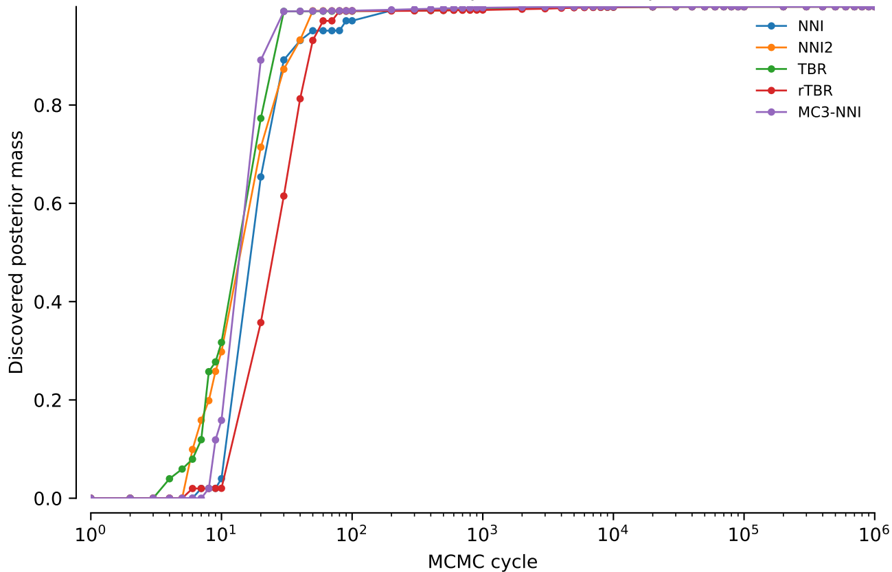
vert.coiii.tw0: Discovered posterior mass: power = 0.1
