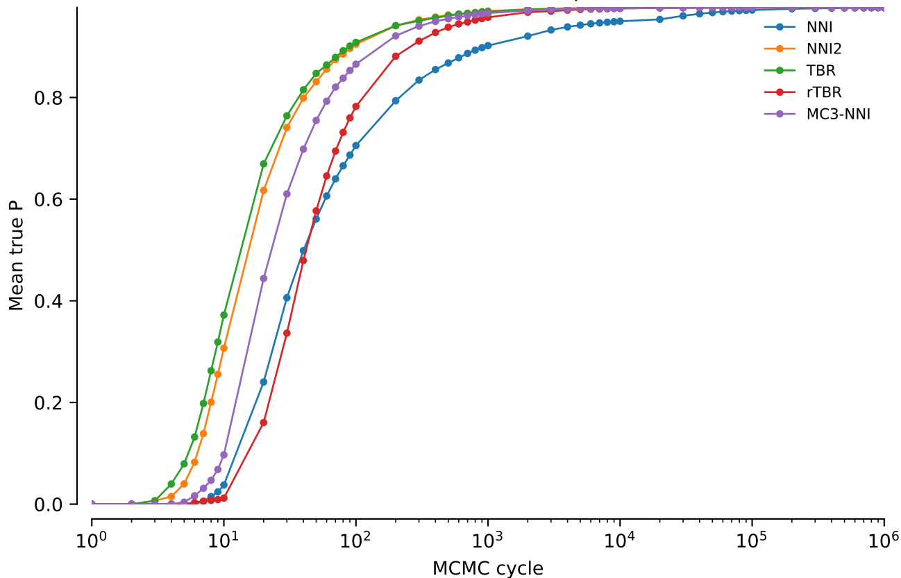
vert.coiii.tw0: Mean true P: power = 0.2
