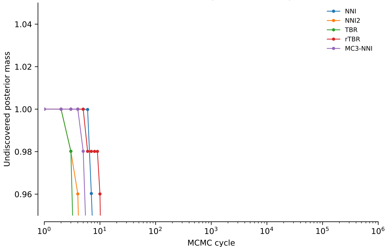
vert.coiii.tw0: Undiscovered posterior mass: power = 0.2
