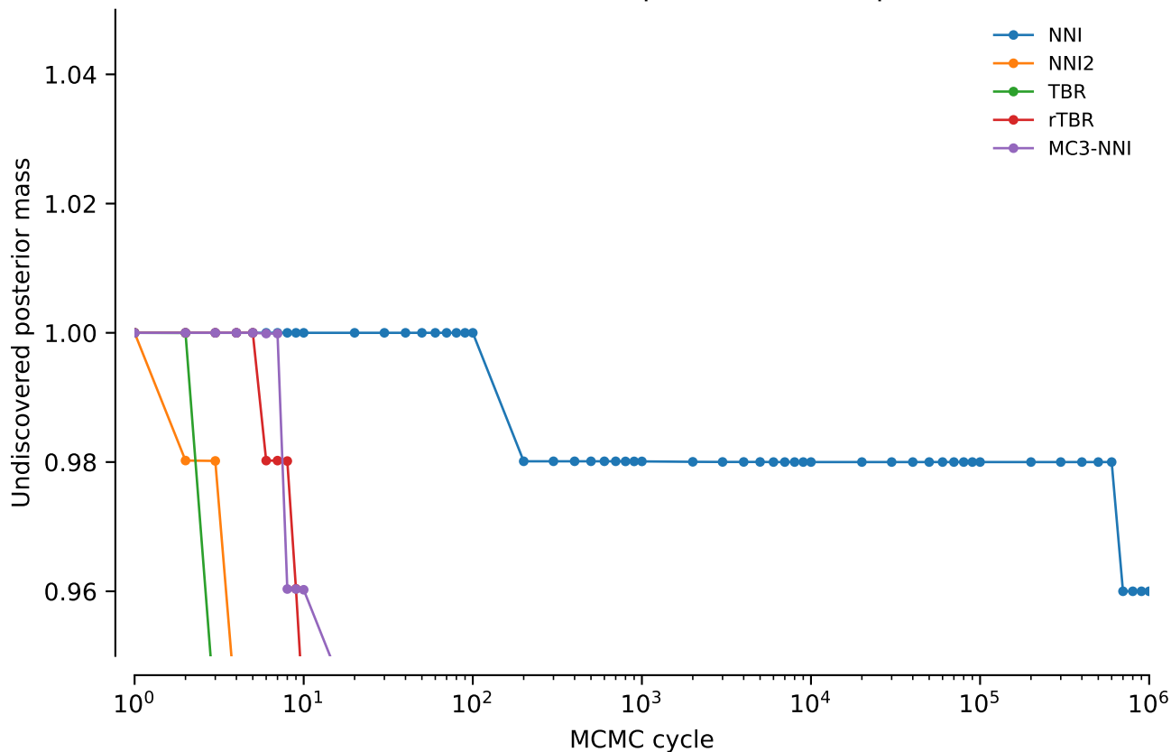
vert.coiii.tw0: Undiscovered posterior mass: power = 0.5
