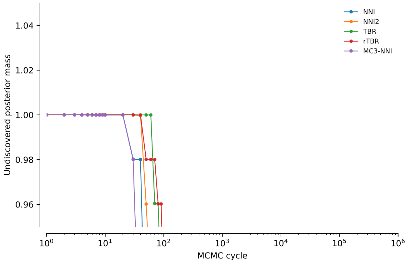
vert.coiii.tw0: Undiscovered posterior mass: power = 0
