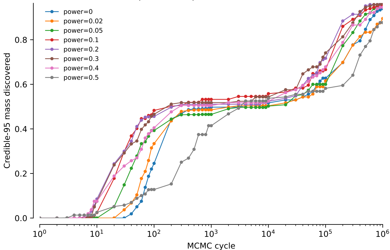
vert.coiii.tw2: NNI power comparison: Credible-95 mass discovered
