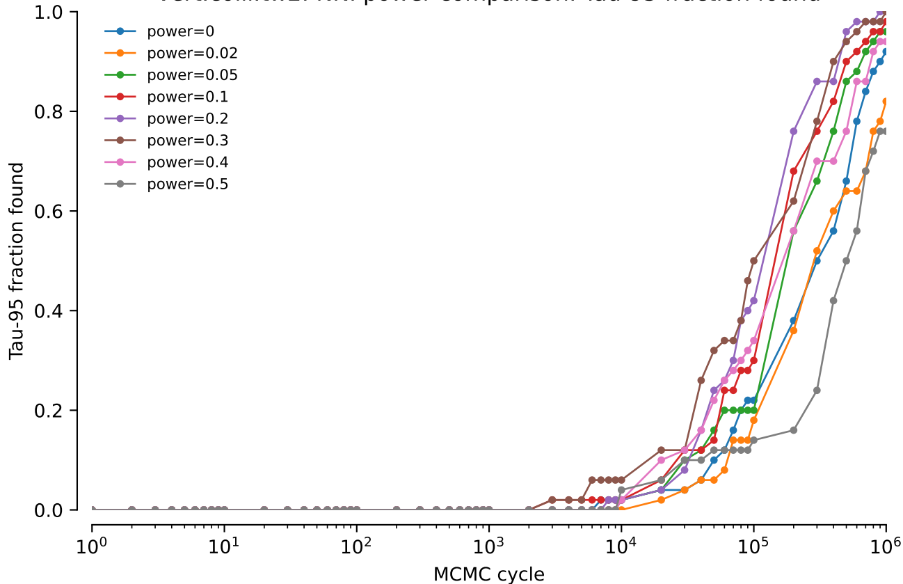
vert.coiii.tw2: NNI power comparison: Tau-95 fraction found
