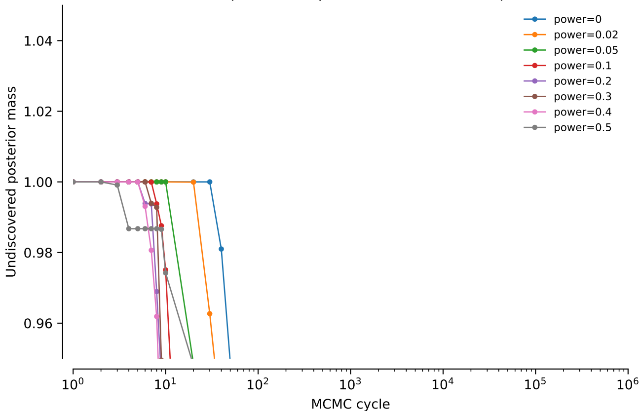
vert.coiii.tw2: NNI power comparison: Undiscovered posterior mass
