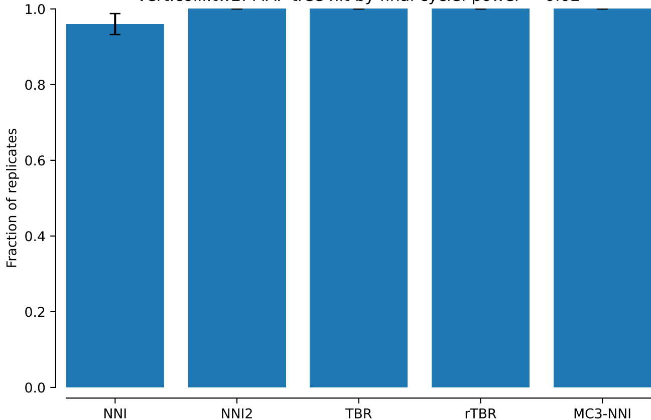
vert.coiii.tw2: MAP tree hit by final cycle: power = 0.02
