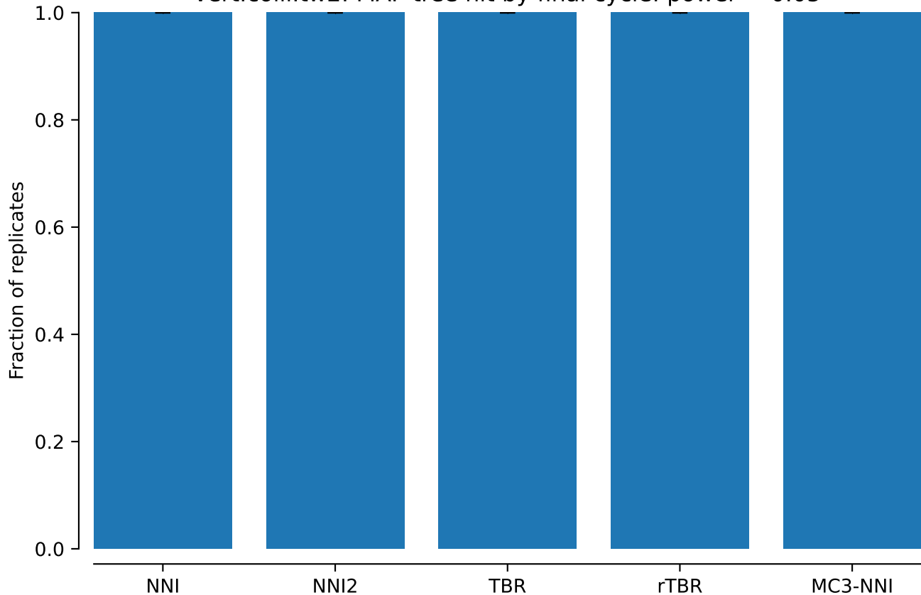
vert.coiii.tw2: MAP tree hit by final cycle: power = 0.05
