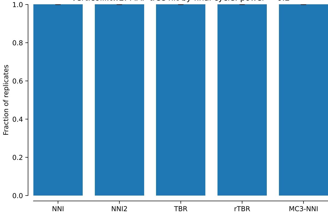
vert.coiii.tw2: MAP tree hit by final cycle: power = 0.2
