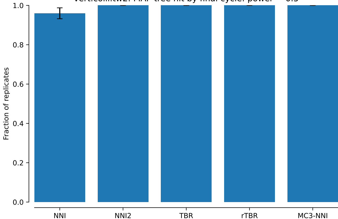
vert.coiii.tw2: MAP tree hit by final cycle: power = 0.5
