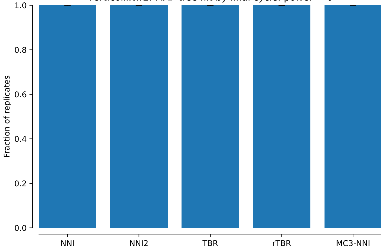
vert.coiii.tw2: MAP tree hit by final cycle: power = 0
