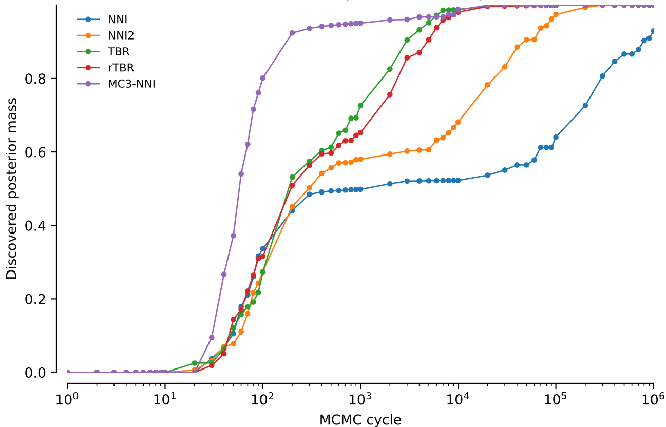
vert.coiii.tw2: Discovered posterior mass: power = 0.02
