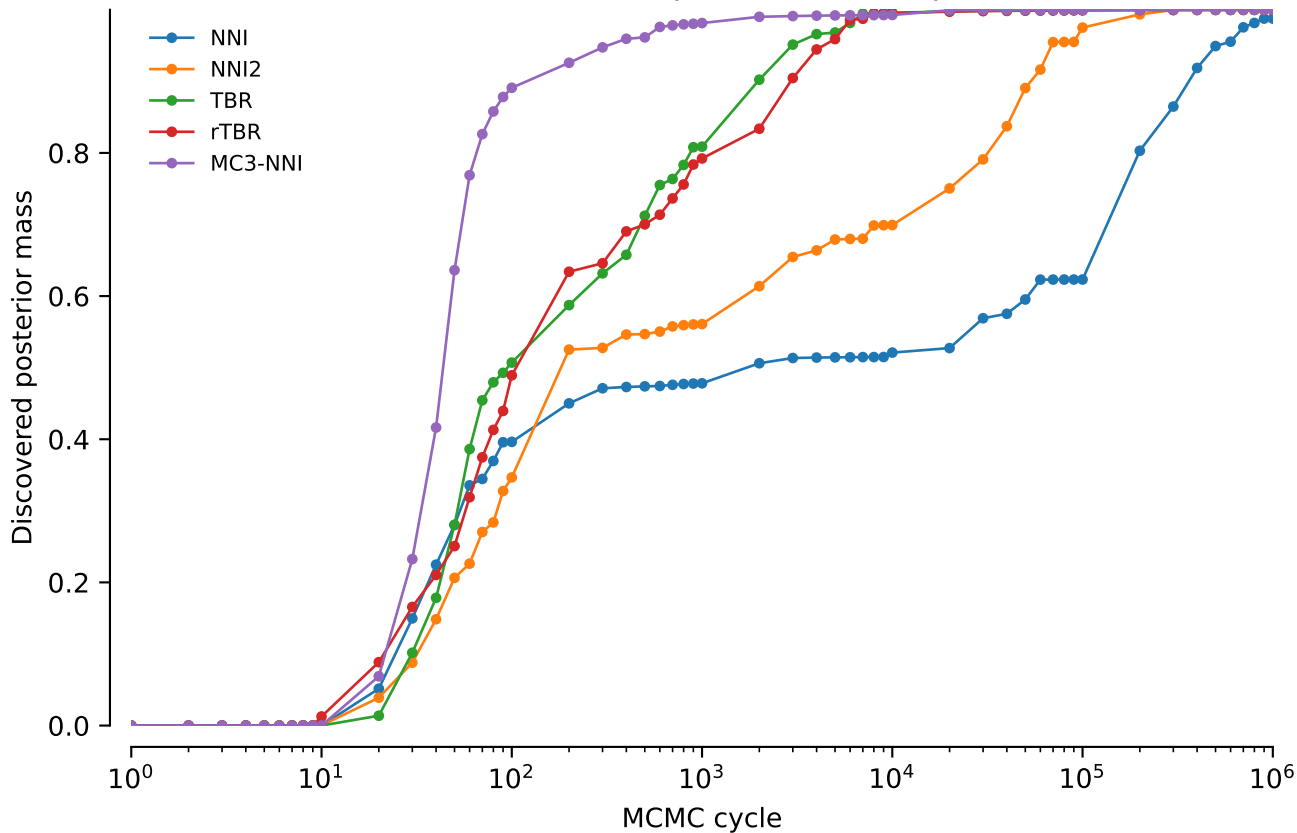
vert.coiii.tw2: Discovered posterior mass: power = 0.05
