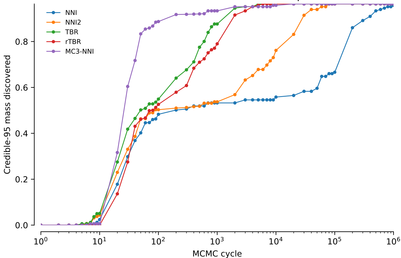
vert.coiii.tw2: Credible-95 mass discovered: power = 0.1
