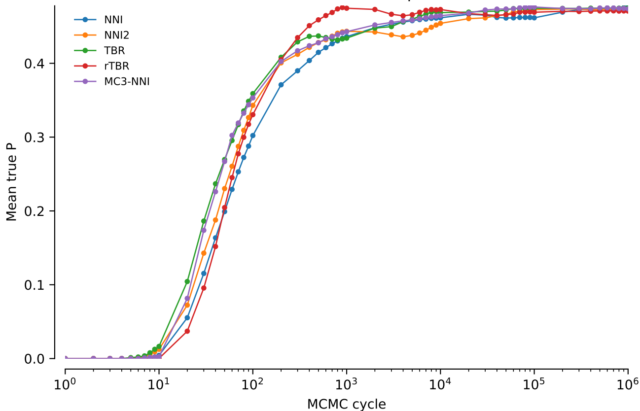
vert.coiii.tw2: Mean true P: power = 0.1
