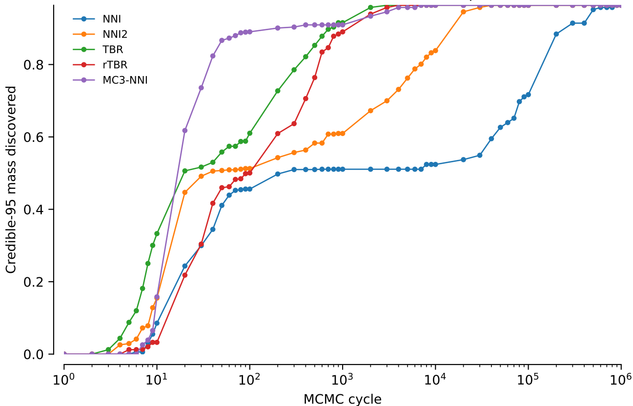
vert.coliii.tw2: Credible-95 mass discovered: power = 0.2
